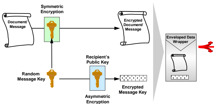
Fig. 4: Digital Envelope
