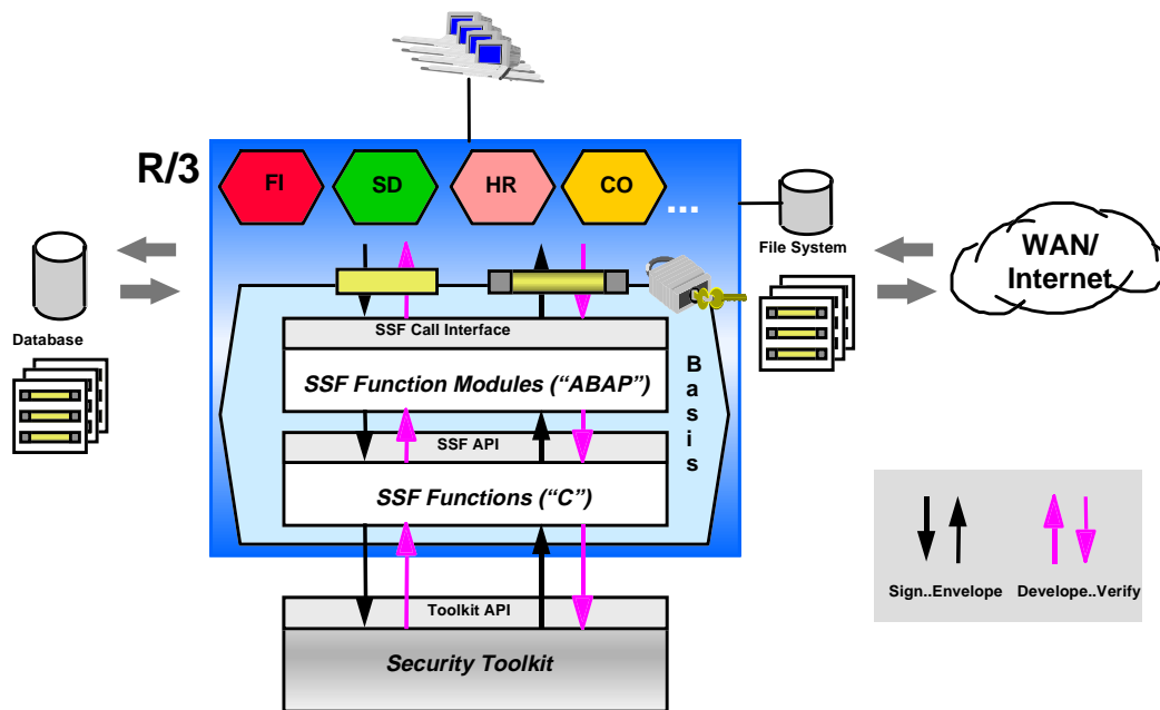
Fig. 5: SSF Architecture
