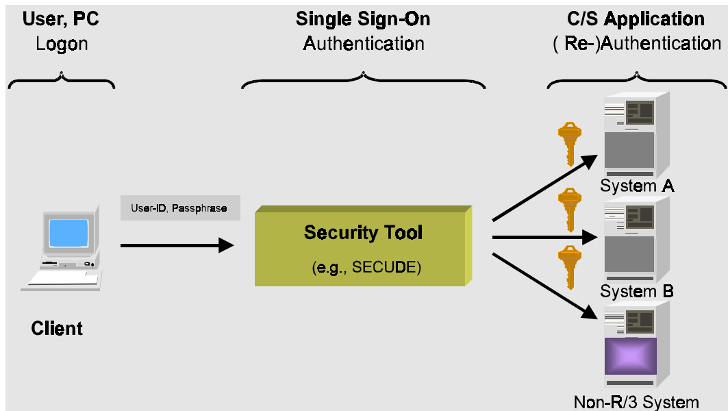
Fig. 1: Single Sign-On
