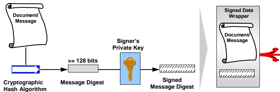
Fig. 3: Digital Signature
